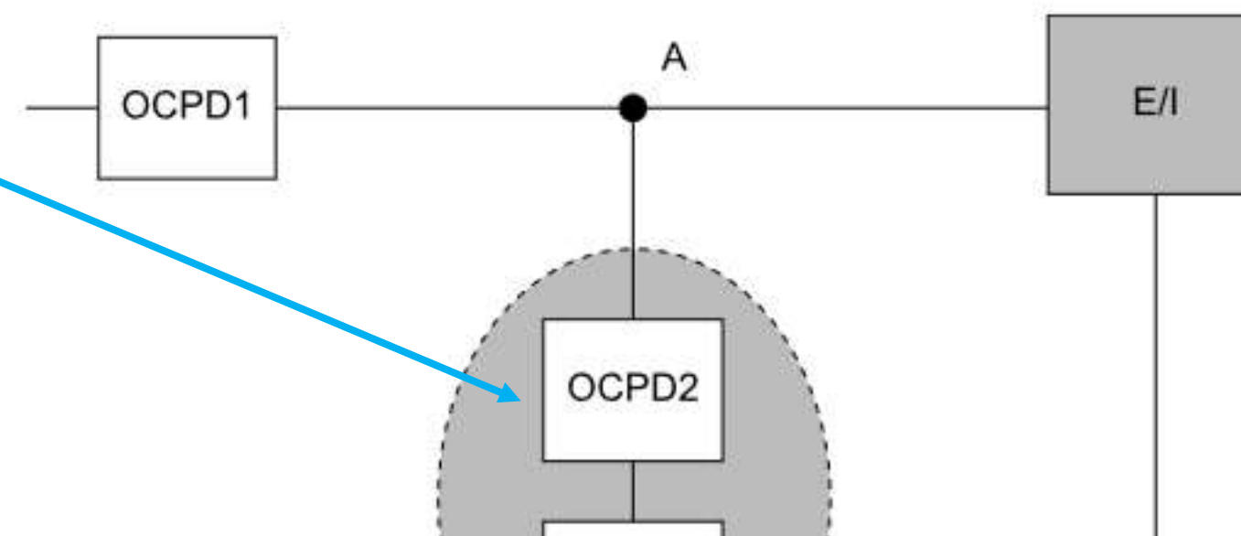
Fig 534.5 – Connection points of an SPD assembly
